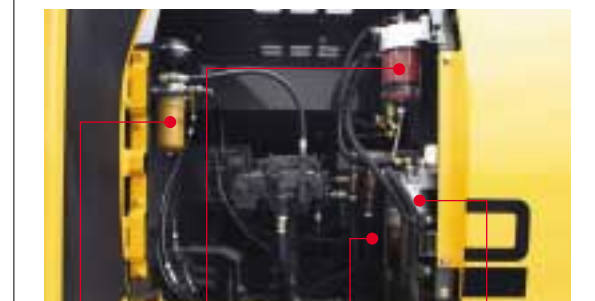
Pilot filter Pre-fuel filter (with water separator) Engine oil filter Main fuel filter (with water separator)
